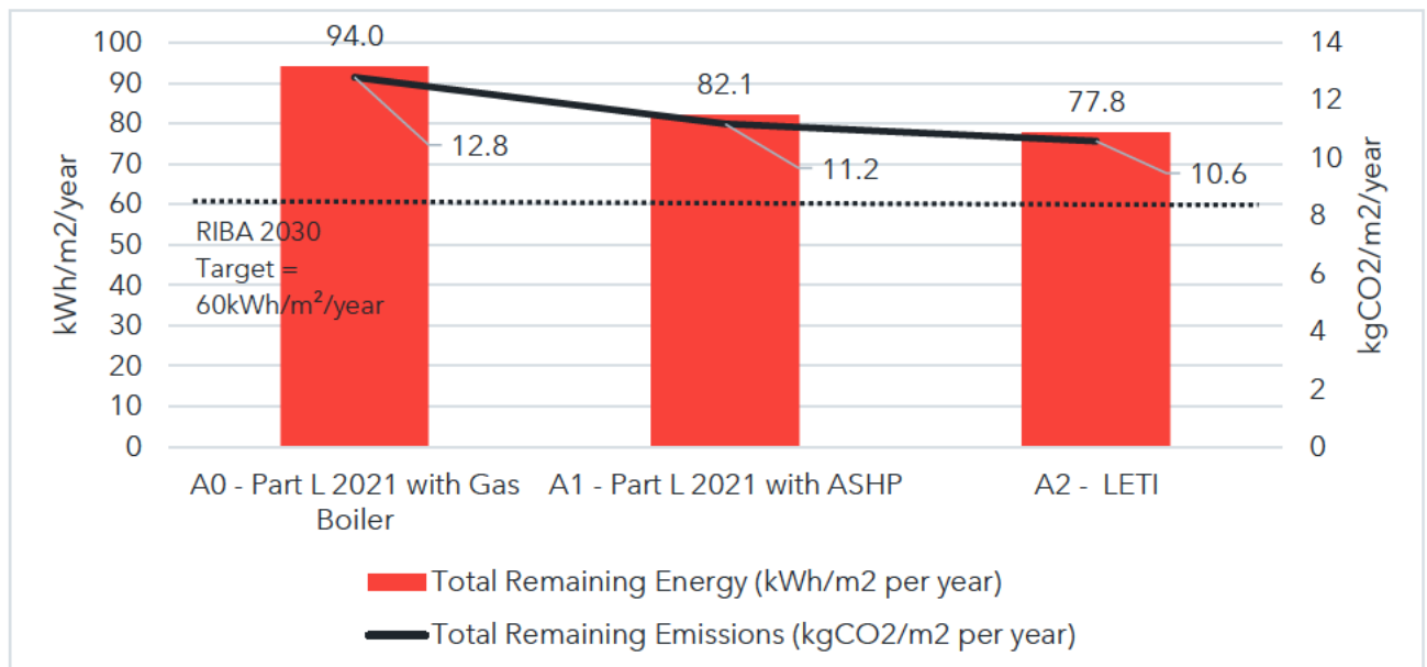
Figure 2.3.1-2 - Office – Total energy consumption and carbon emissions after all on-site measures, excluding rooftop PV generation, are applied, presented per policy approach and compared against RIBA 2030 operational energy targets for non-domestic
