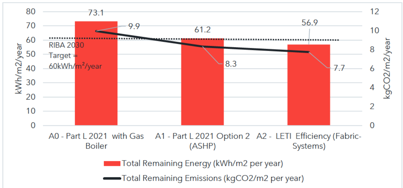
Figure 2.3.1-3 - Office – Total energy consumption and carbon emissions after all on-site measures, including rooftop PV generation, are applied, presented per policy approach and compared against RIBA 2030 operational energy targets for non-domestic
