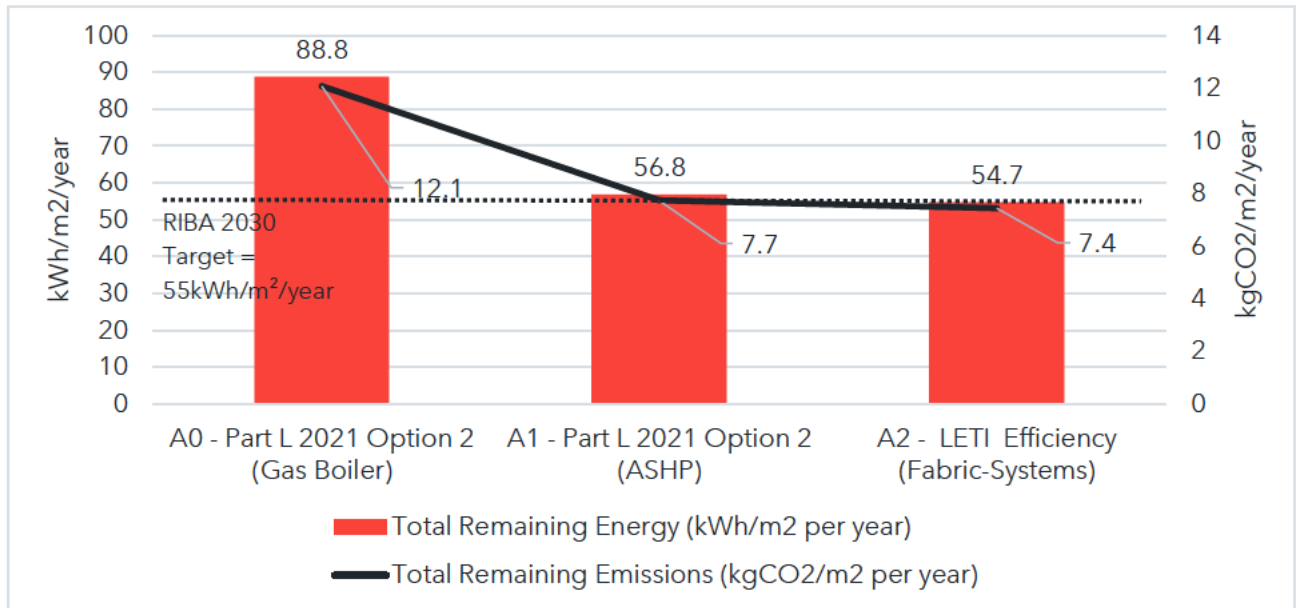
Figure 2.3.2-5 - School – Total energy consumption and carbon emissions after all on-site measures, including rooftop PV generation , are applied, presented per policy approach and compared against RIBA 2030 operational energy targets for non-domestic
